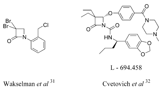
Scheme 4. Reference compounds.
