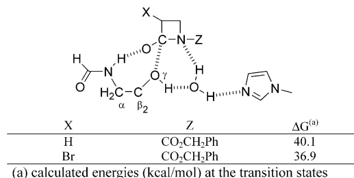
Figure 3. Theoretical evaluation of nucleophilic attack in a model of elastase active site.
