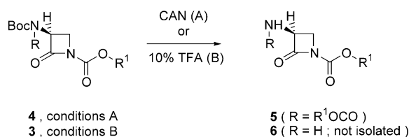
Scheme 2. Deprotection of compounds 3–4.
