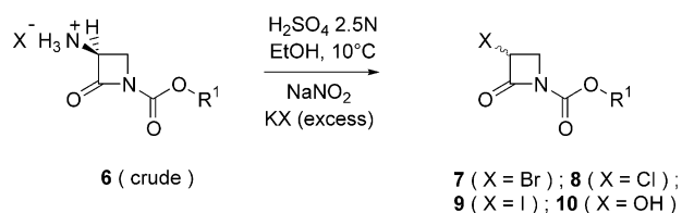
Scheme 3. Synthesis of compounds 7–10.
