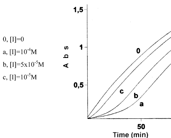
Figure 2. Inhibition of PPE.
