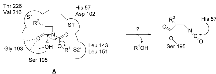
Figure 1. Expected mechanism of suicide-inhibition of elastase.
